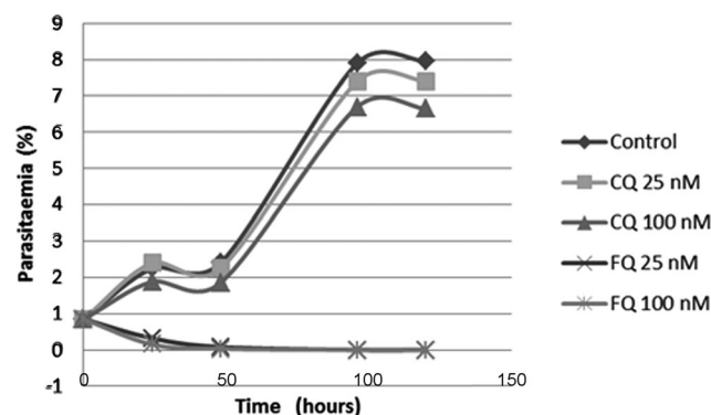
Figure 5. Evolution of the parasitaemia as a function of time of cultures of synchronized parasites at the trophozoite-schizont stages of the CQ-resistant strain FcB1 pretreated during 5 h with 25 and 100 nM FQ and CQ, or in the absence of drug (control).
