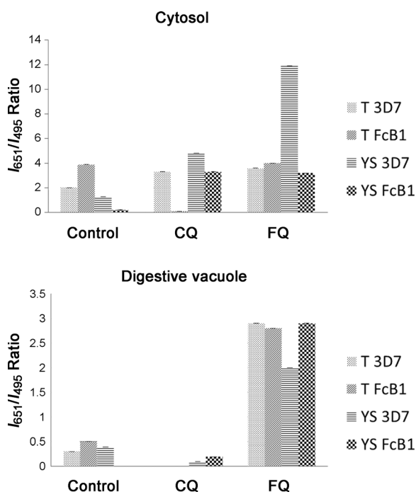
Figure 4. Quantification of the I_{651}/I_{495} ratio in the cytosol (top) and the digestive vacuole (bottom) of P. falciparum parasites (CQ-susceptible strain 3D7 and CQ-resistant strain FcB1) without drug (control) or after drug treatment (CQ or FQ) at the trophozoite (T) and young schizont (YS) stages.
