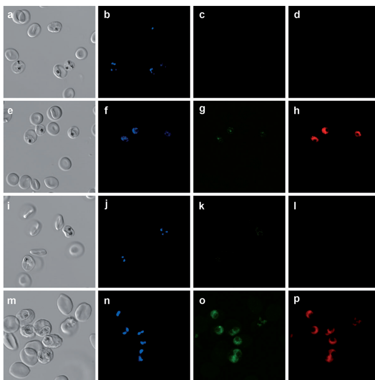
Figure 3. a)–d) Red blood cells infected by the CQ-susceptible strain (3D7) pre-treated by FQ (40 nM, 30 min), fixed and stained with DAPI; e)–h) red blood cells infected by the CQ-susceptible strain (3D7) pre-treated by FQ (40 nM, 30 min), incubated with 1 (40 \mu\text{M} for 5 min), fixed and stained with DAPI; i)–l) red blood cells infected by the CQ-resistant strain (FcB1) pre-treated by FQ (40 nM, 30 min), fixed and stained with DAPI; m)–p) red blood cells infected by the CQ-resistant strains (FcB1) pre-treated by FQ (40 nM, 30 min), incubated with 1 (40 \mu\text{M} for 5 min), fixed and stained with DAPI. Bright-field images (a, e, i, m) and corresponding DAPI fluorescence emission (b, f, j, n), green fluorescence emission (c, g, k, o), and red fluorescence emission (d, h, l, p).
