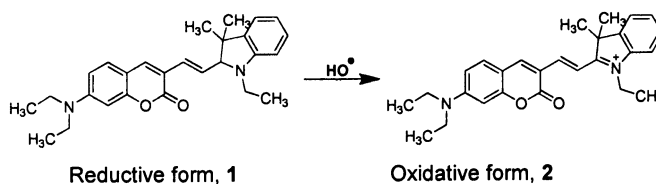
Figure 2. Ratiometric fluorescent probe with high selectivity for hydroxyl radicals.
